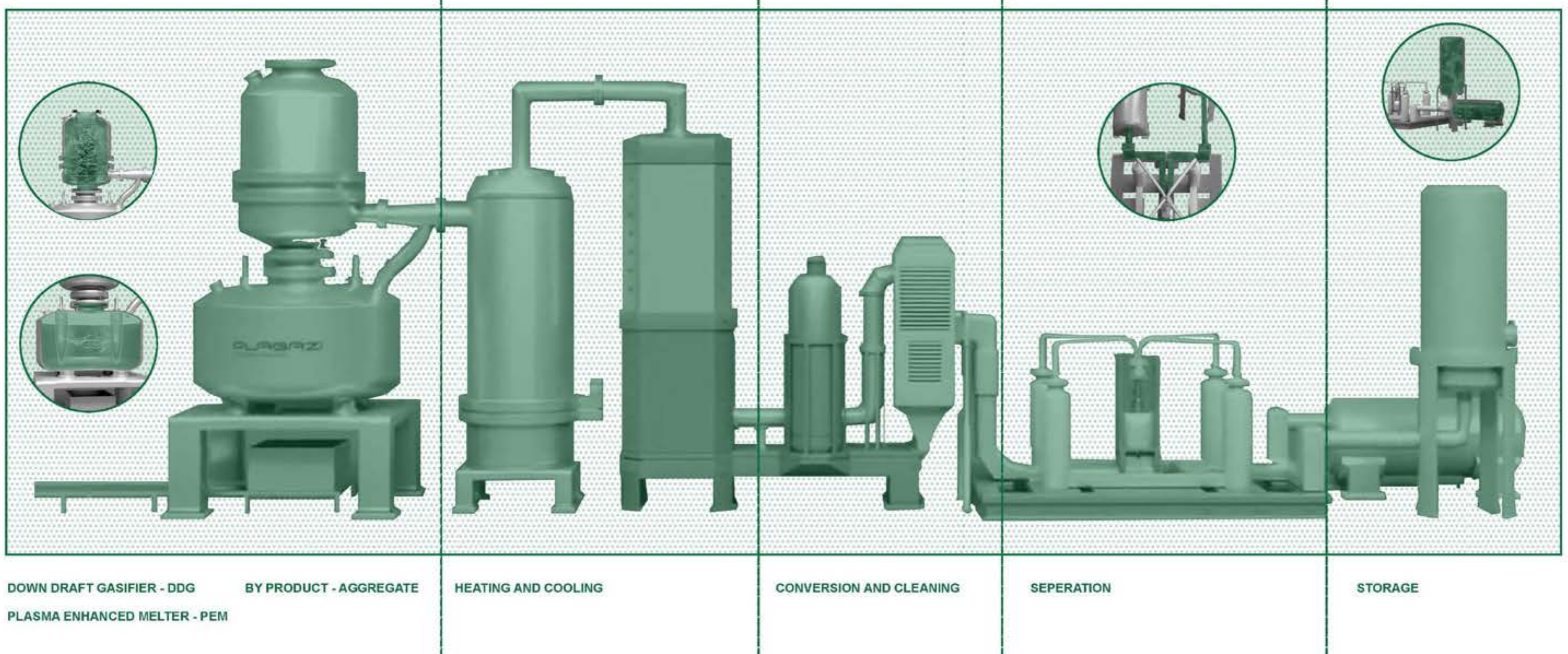
HTE PROCESS Waste converted to Hydrogen and Carbon Dioxide
